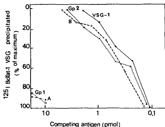
Fig.3. Inhibition of the cross-reaction ^{125}\text{I} -BoTat-1 VSG versus anti-BoTat-28 VSG by native BoTat-1 VSG, tryptic fragment A (▲-▲) and B (○-○) and proteinase K glycopeptides Gp1 (□-□) and Gp2 (Δ-Δ).
